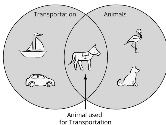
Figure 8.6 A Simple Venn Diagram Showing Sets and Subsets
